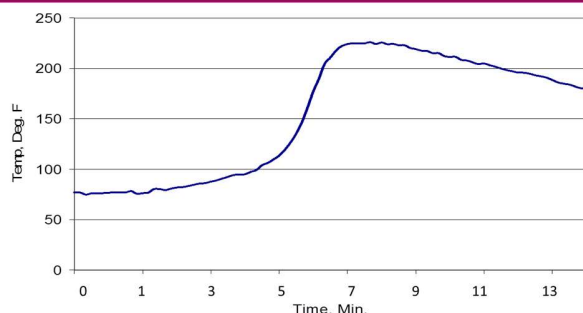
Typical Exotherm Curve at 74°F (10 grams) at 10:1 mix ratio by volume 5
